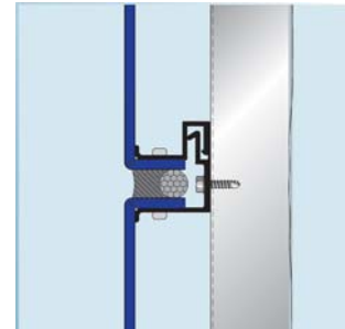
vertical section
