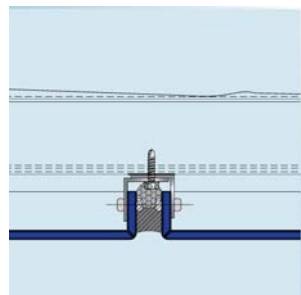
horizontal section
