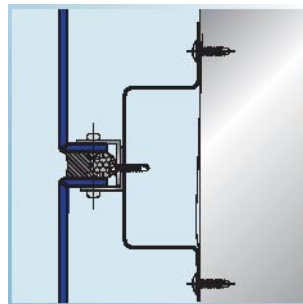
vertical section
