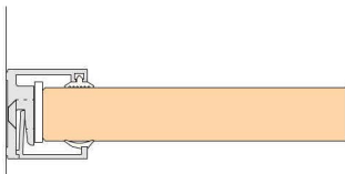
MRC 29 Frame profile for panels up to 19 mm
