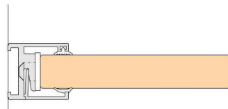
MRC 35 Frame profile for panels up to 19 mm
