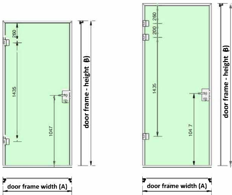
ATC 45 frame with 2 hinges, lock casing + handle set
