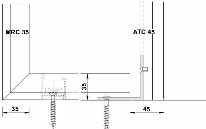
MRC 35 frame and ATC 45 door frame
