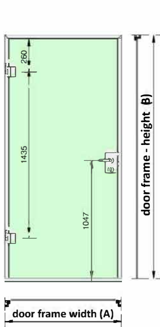
ATC 45 frame with 2 hinges, lock casing + handle set
