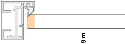
ATC 45 Wall fixed door frame profile
