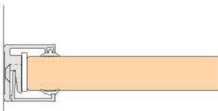
MRC 29 Frame profile for panels up to 19 mm
