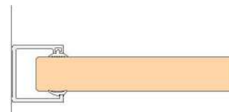
Profile No. 594 Frame profile for panels up to 19 mm
