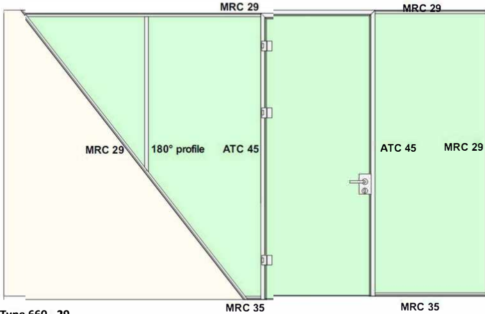
Type 660 - 29 freestanding door frame with ceiling connection
