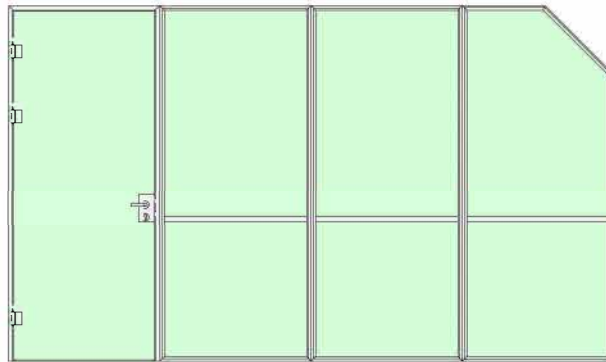
ATC 45 door frame with door and frame combinations MRC 35
