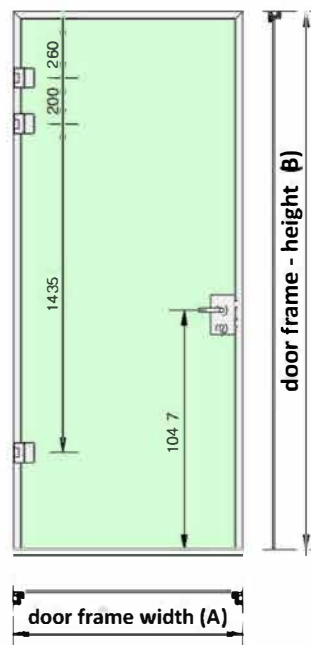
ATC 45 frame with 3 hinges, lock casing + handle set
