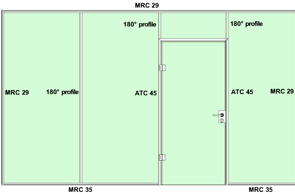
Type 650 - 29 freestanding door frame with ceiling connection
