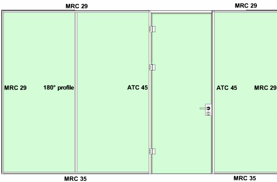
Type 660 - 29 freestanding door frame with ceiling connection
